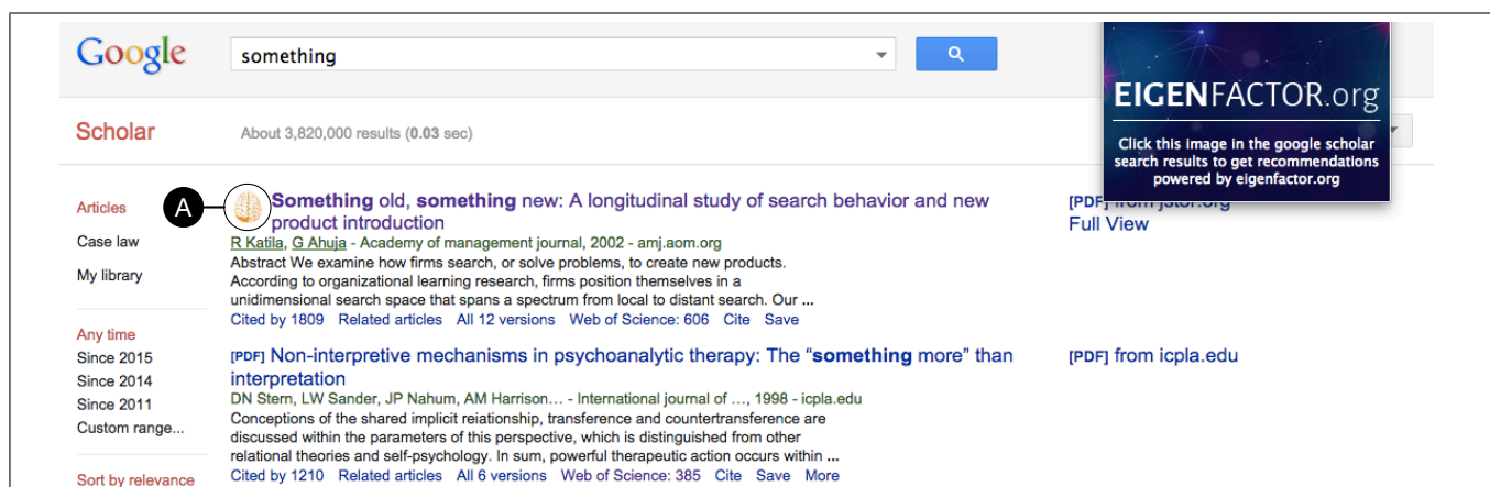
Figure 3: Screenshot of our browser plugin (Chrome or Firefox), which provides recommendations directly on the Google Scholar site. The plugin scrapes the titles of a search result and looks them up in Babel. If Babel has recommendations for this title a small brain icon (A) is inserted next to the result. Clicking this icon takes you to the Babel demonstration website (Figure 2), where recommended papers are displayed.
